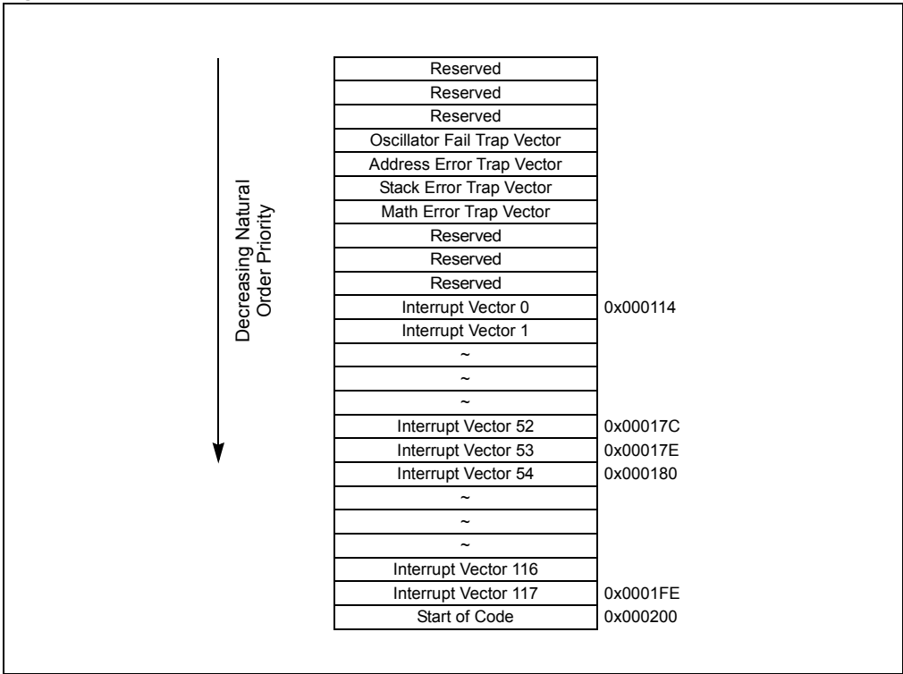
Figure 1-2: Fixed Location Alternate Interrupt Vector Table (AIVT)
