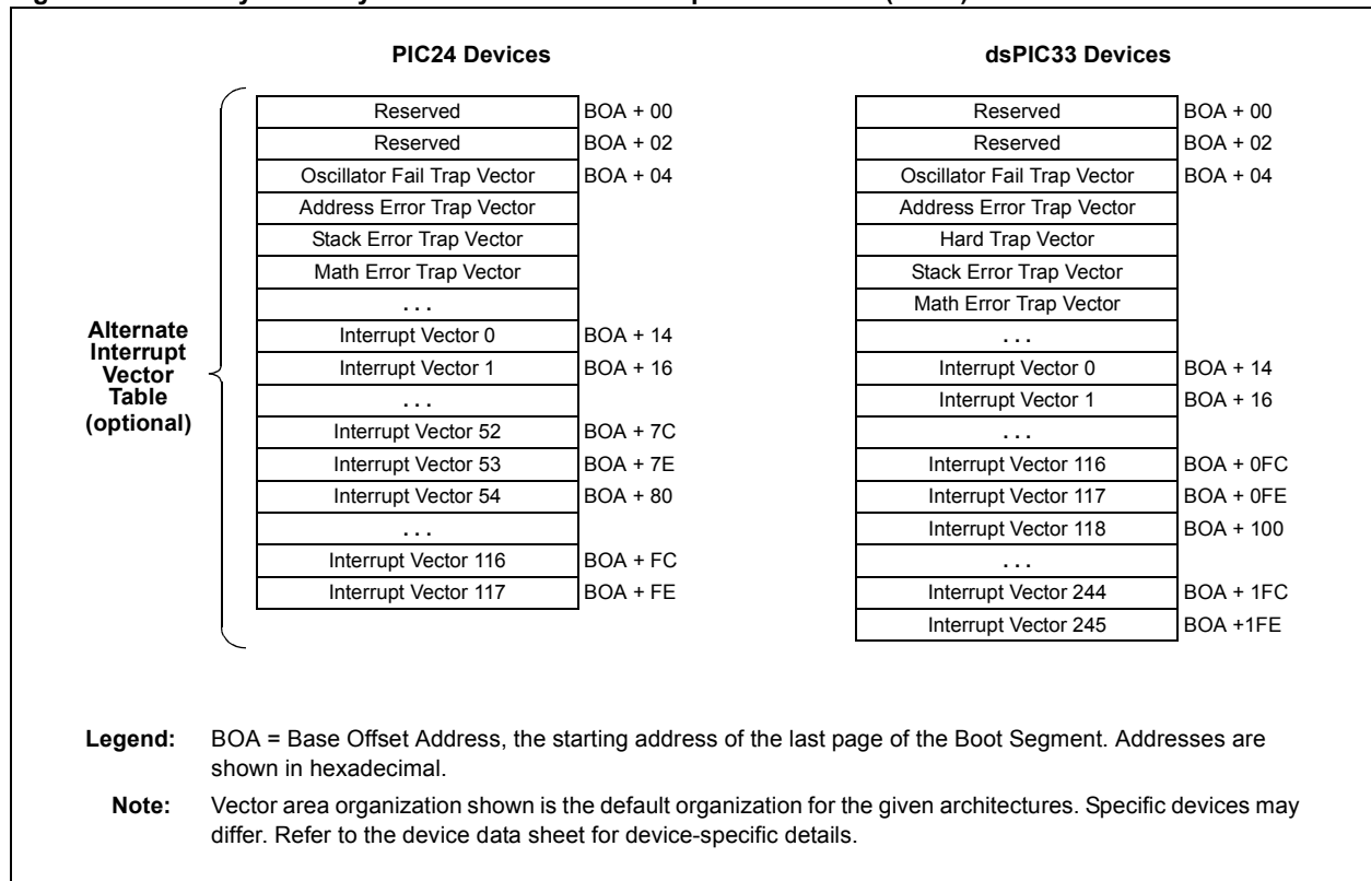
Figure 1-3: Dynamically Located Alternate Interrupt Vector Table (AIVT)
