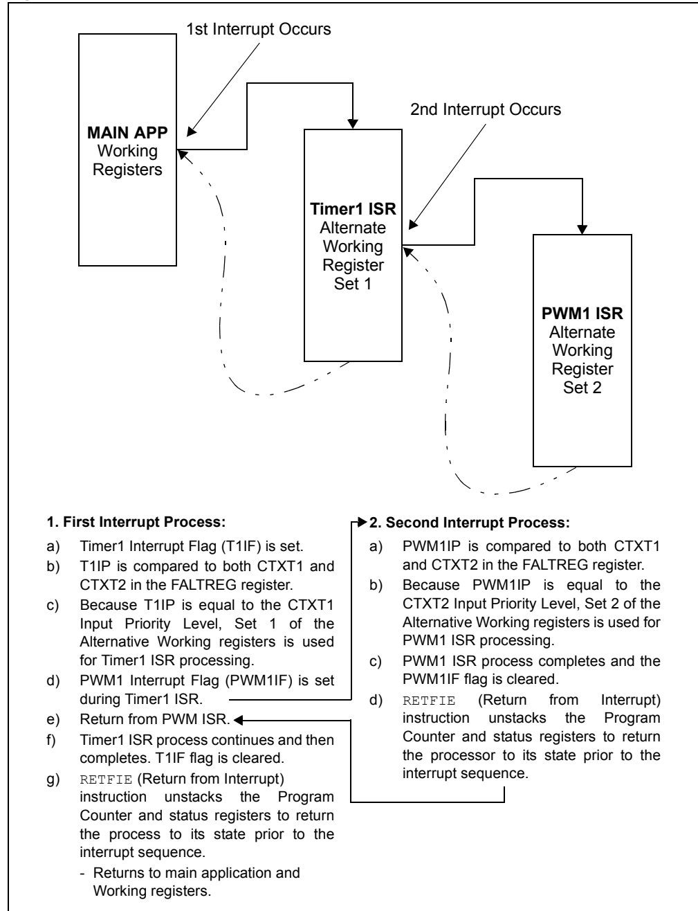
Figure 3-2: Nested Interrupt Sequence
