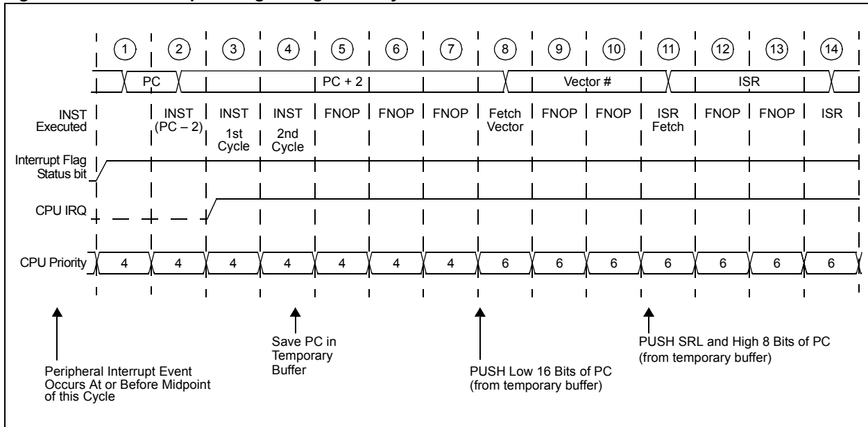
Figure 4-2: Interrupt Timing During a Two-Cycle Instruction
