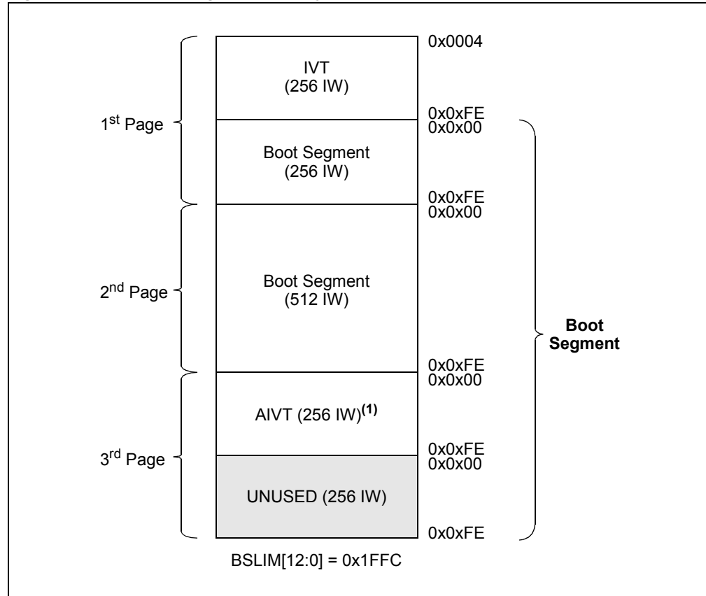
Figure 1-4: Boot Segment Memory and AIVT Implementation
