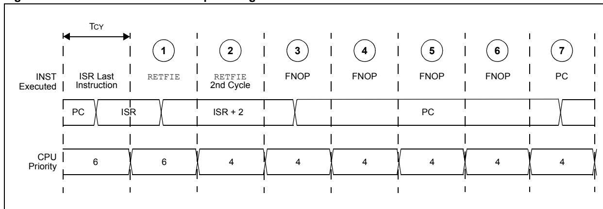
Figure 4-4: Return from Interrupt Timing
