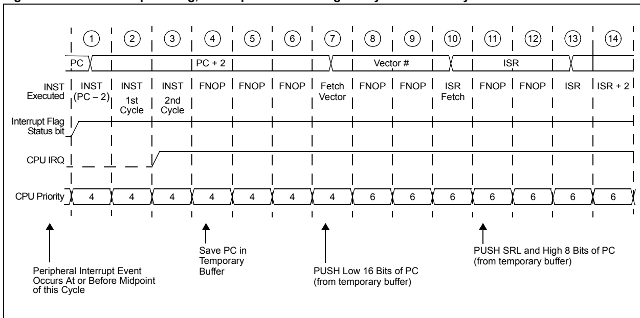
Figure 4-3: Interrupt Timing, Interrupt Occurs During 1st Cycle of a Two-Cycle Instruction
