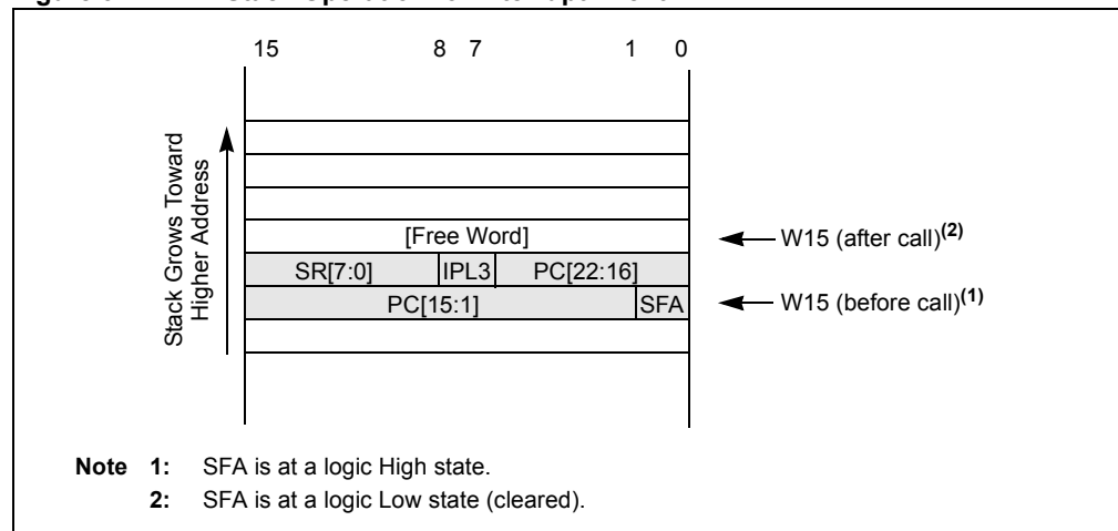
Figure 3-1: Stack Operation for Interrupt Event
