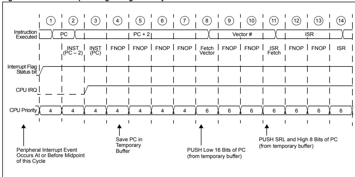
Figure 4-1: Interrupt Timing During a One-Cycle Instruction
